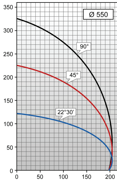
Cutting charts
